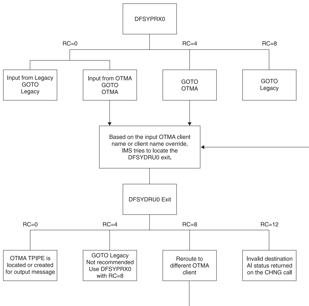
Figure 29. How DFSYPRX0 and DFSYDRU0 Determine Message Destination
