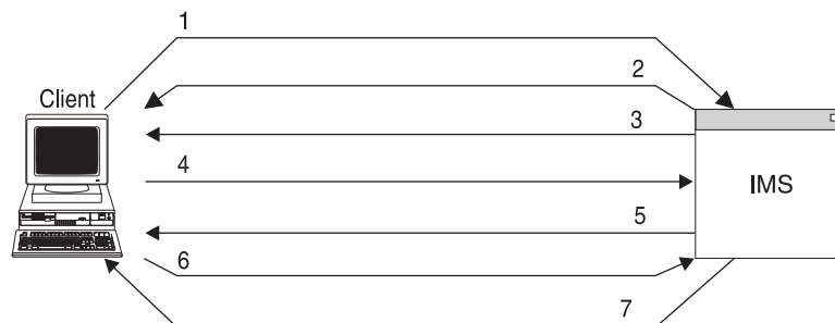
Figure 19. Flow of Resynchronization (Nondeferred)
