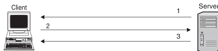
Figure 17. Server-Available Flow
