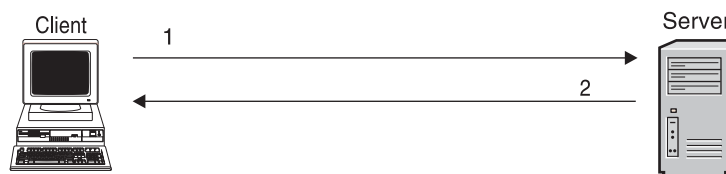
Figure 16. Client-Bid Flow
